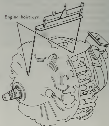
FIGURE 8-10. Engine showing hoisting sling attached.
